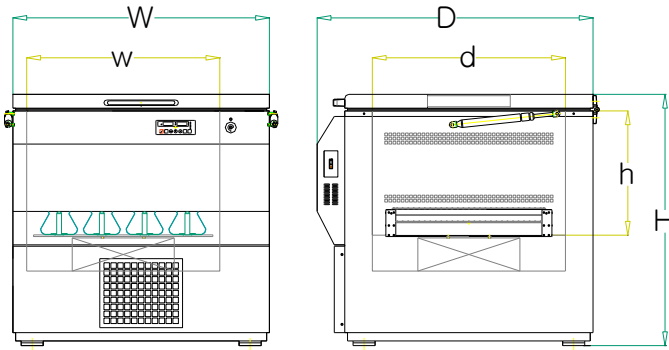
**Shaking Incubator, Dimensions DK-SIF220
